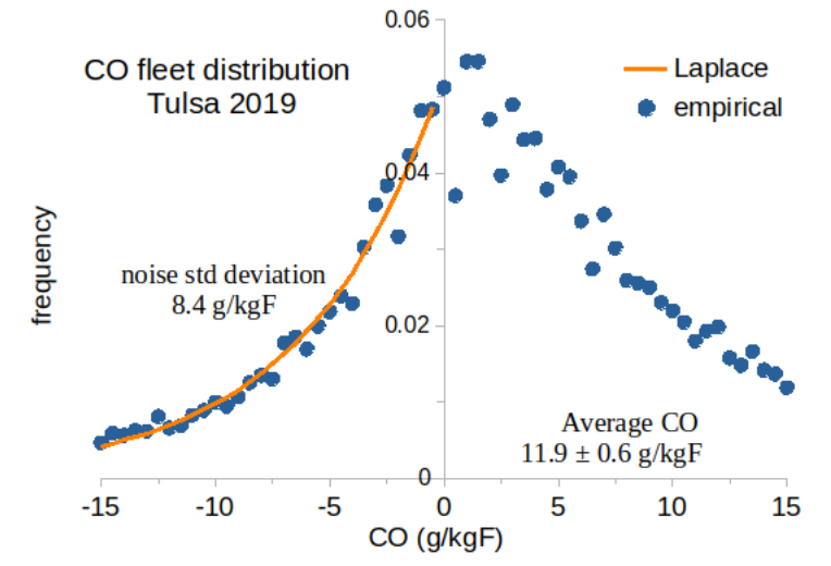
Figure 3. RSD signal plus noise for CO. Points represent the empirical distribution. The line is a fit of the Laplace distribution to the negative data points.
